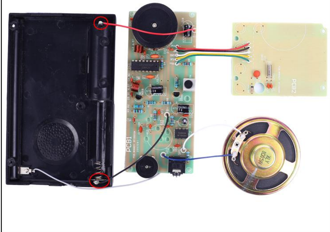
Step 38: Connect 80mm Red wire to Positive Metal Sheet and connect 80mm Black wire to Negative Metal Sheet(with Spring).
